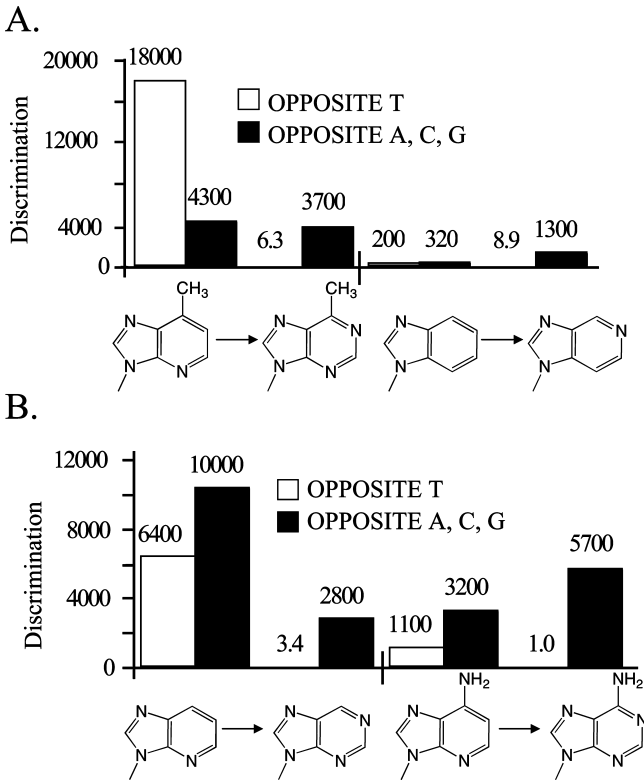
FIGURE 4: Effect of adding N-1 to 1-deaza-6-methylpurine and benzimidazole (panel A), and 1-deazapurine and 1-deazaadenine (panel B). The DF for polymerization opposite T and the average DF for polymerization opposite A, C, and G are shown.
