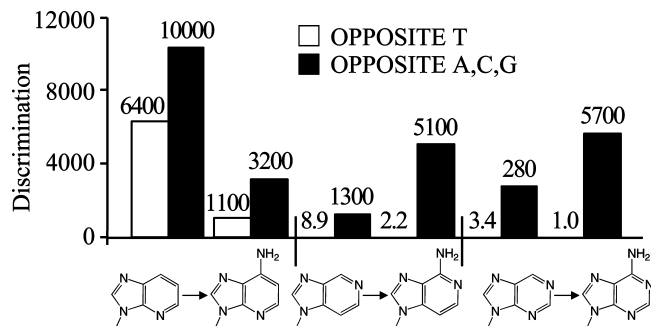
FIGURE 5: Effect of adding N 6 to 1-deazapurine, 3-deazapurine, and purine. The average DFs (opposite A, C, and G) for T are shown.
