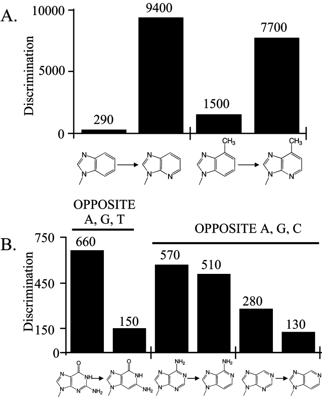
FIGURE 3: Effects of adding N-3 to low-fidelity bases and removing N-3 from high-fidelity bases. Panel A shows the effect of adding N-3 to benzimidazole and 4-methylbenzimidazole on the average DF for polymerization opposite A, T, C, and G. Panel B shows the effect of removing N-3 from guanine, adenine, and purine for misincorporation opposite either A, G, and T (dGTP/d3DGTP) or A, G, and C (dPTP/d3DPTP and dATP/d3DATP).
