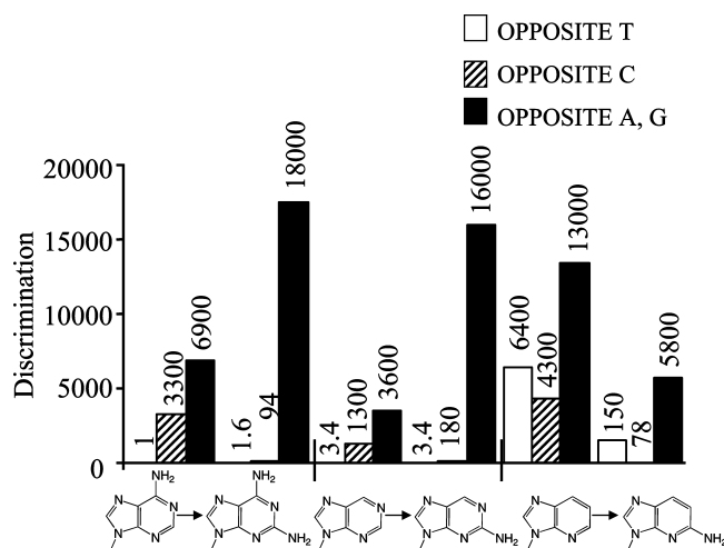
FIGURE 6: Effect of adding N 2 to adenine, purine, and 1-deazapurine. The values of the average DFs (opposite A and G), along with those opposite T and C, are shown.
