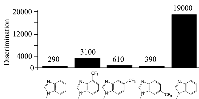
FIGURE 2: Misincorporation frequency of benzimidazole and trifluoromethylbenzimidazole compounds. The values of the average DF (opposite all four DNA templates) are provided.
